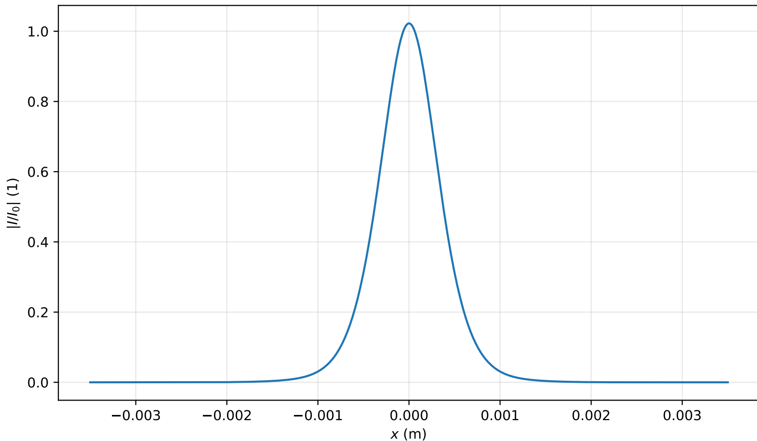
Intensity profile I(x, y = 0, z = 2.309m)/I_0 , P_{in}=0.7P_{cr} , artificial time
